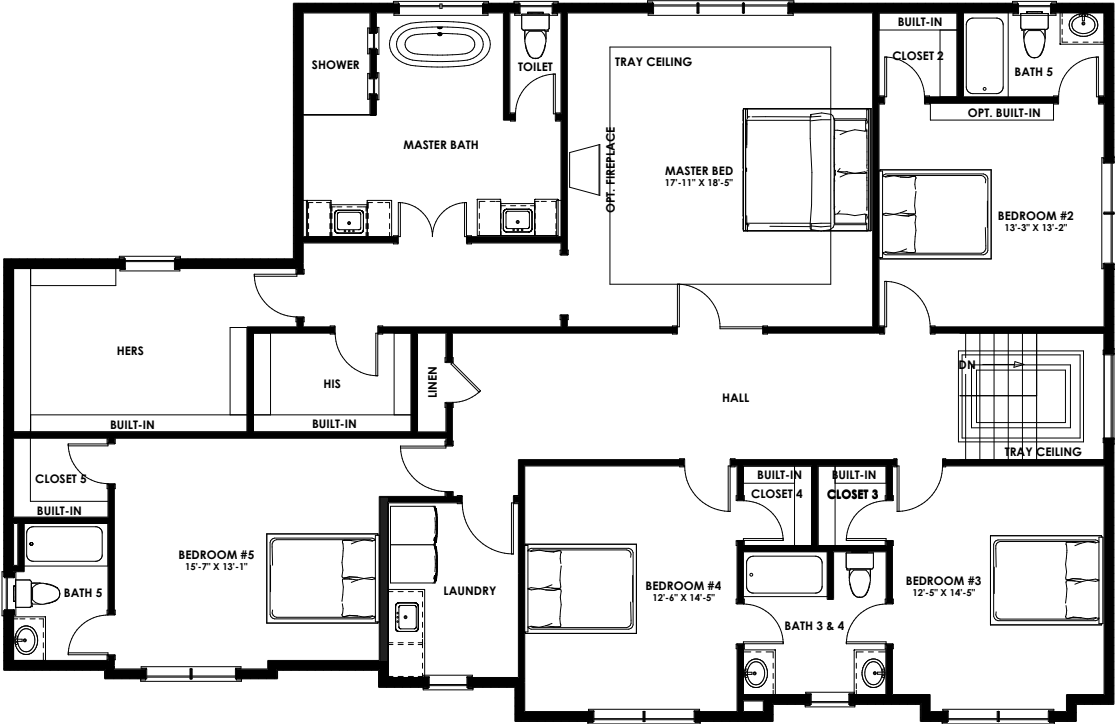
UPPER LEVEL 2,320 SQ FT
